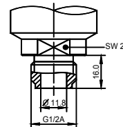
G 1/2 A
