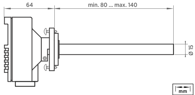
GMD20 Dimensions
