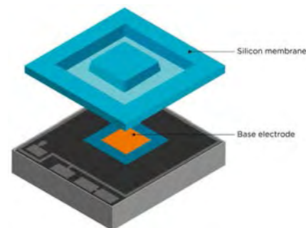
BAROCAP sensor
