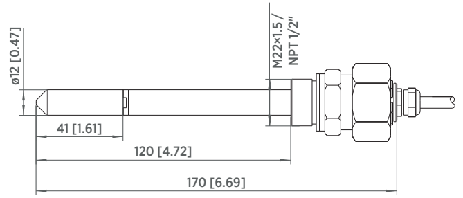
HMT314 Probe
