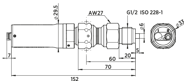
DPT145 with Alstom connector
