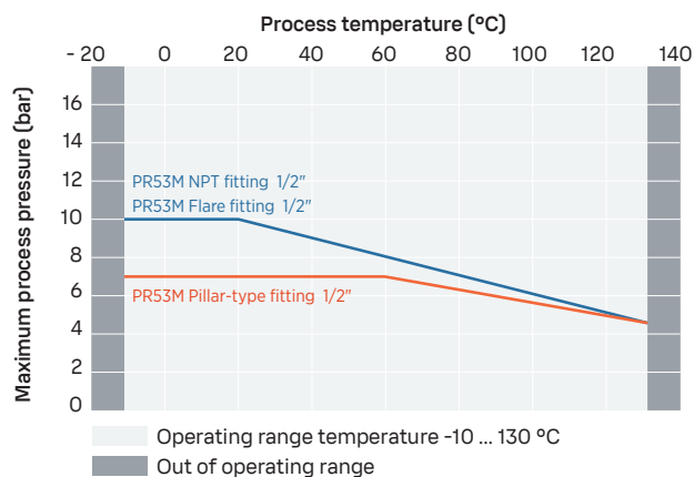
PR53M process pressure
