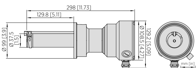
Dimensions of PR53GP L coupling 88.9 mm (3.5 in)
