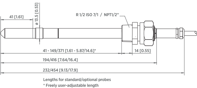
HMT318 Probe
